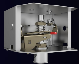
MRM- Mechanical Release Module
