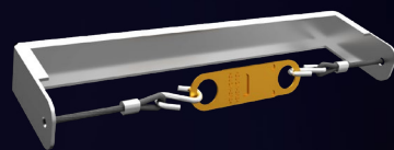
Detector Bracket - Fusible link
